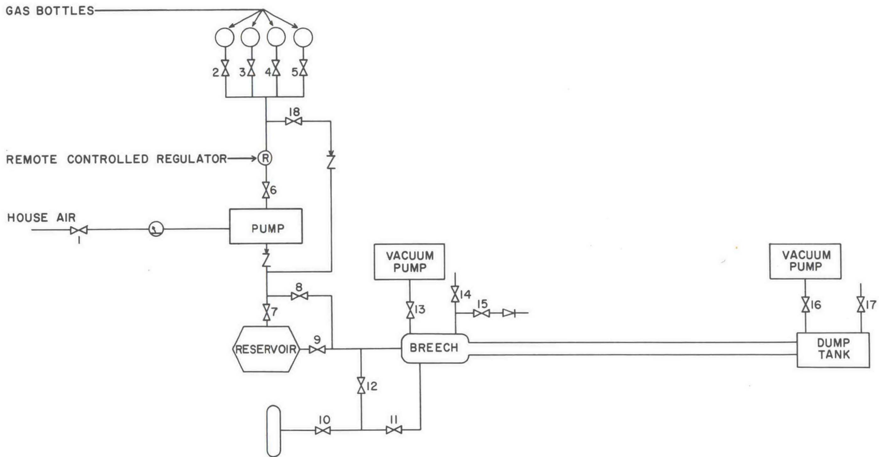
Fig. 13. Gas flow circuit.
